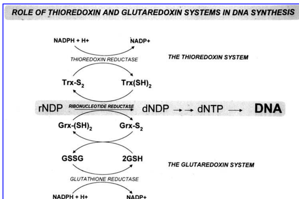
FIG. 1. The principal components of Grx and Trx systems. This slide, made in the 1980s by Dr. Holmgren, schematically shows the Grx and Trx systems as alternative reductants of ribonucleotide reductase, clearly illustrating the glutathione dependence of Grx but with both systems ultimately being propelled by NADPH through either TrxR or glutathione reductase. Trx, thioredoxin; TrxR, thioredoxin reductase; Grx, glutaredoxin; GSH, glutathione; GSSG, glutathione disulfide. (Slide kindly provided by Dr. Holmgren.)
